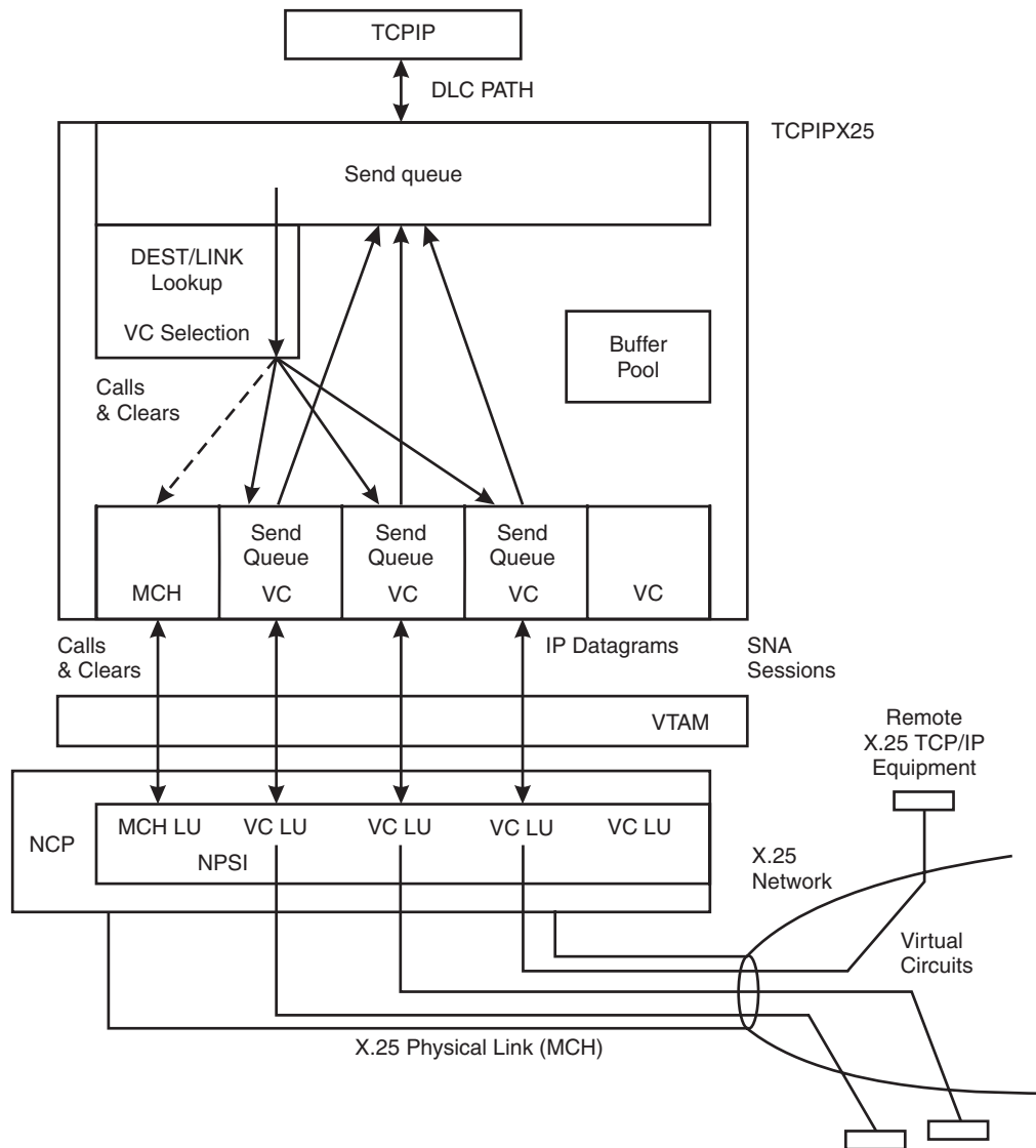
Figure 103. X.25 NPSI environment
